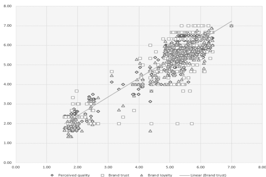
Figure 3: Scatter plot of the correlation analysis Source: Developed for this research
